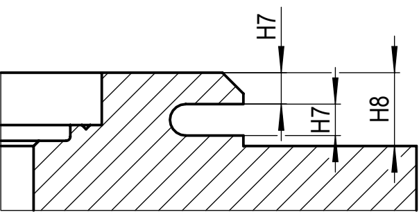
DETAIL X
