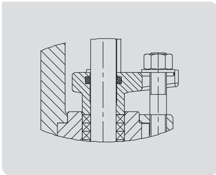
GASKET WITH SCRAPER RING
