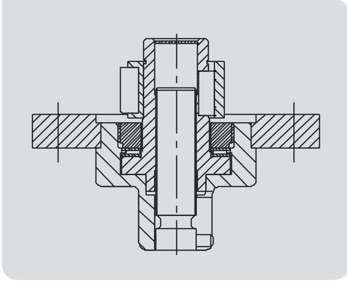
LOCKING DEVICE
